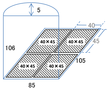
0.8m 3 Gas Kiln
